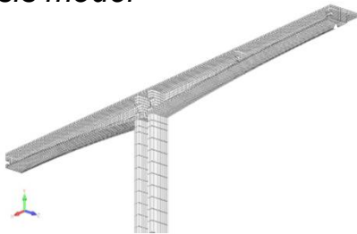
Analysis model
